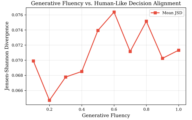
Figure 2: JSD as a function of generative fluency at fixed reasoning depth. The weak positive slope indicates fluency contributes minimally to human-like alignment.
