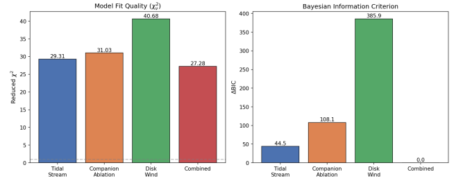
Figure 2: Model comparison showing reduced \chi^2 (left) and \Delta\text{BIC} (right) for each model. The combined tidal+companion model is statistically preferred.
