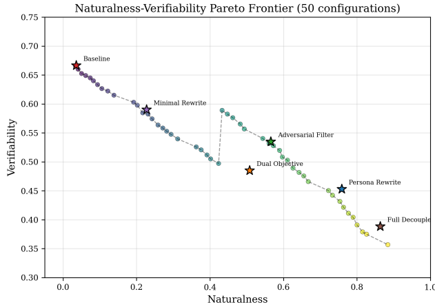
Figure 2: Naturalness-verifiability Pareto frontier from 50 swept configurations. Named strategies are marked with stars.
