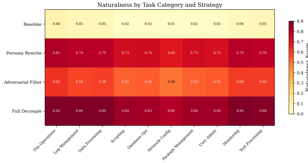
Figure 3: Naturalness scores by task category and conditioning strategy. Warmer colors indicate higher naturalness.
