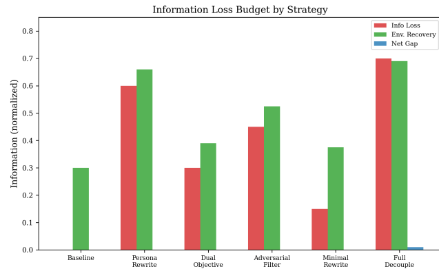
Figure 5: Information loss budget showing specification loss, environment recovery, and net information gap for each strategy.
