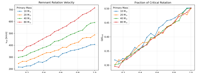
Figure 2: Remnant rotation velocity (left) and fraction of critical rotation (right) vs mass ratio.
