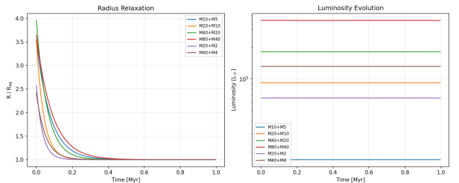
Figure 4: Post-merger thermal relaxation: radius (left) and luminosity (right) evolution.
